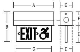
Recess Wall
